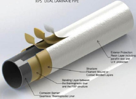
RPS DUAL LAMINATE PIPE
